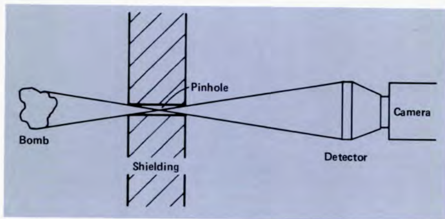
Schematic of a pinhole imaging experiment.
